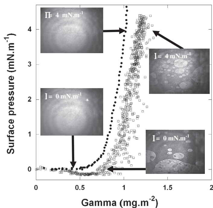
Fig. 1. Surface pressure ( \Pi ) versus surface concentration ( \Gamma ) for the lowest subphase concentrations for which the surface pressure is initiated: 1 \mu\text{g.mL}^{-1} for ovotransferrin in citrate (open squares) and 3 \mu\text{g.mL}^{-1} in acetate (filled circles). The insert in the BAM pictures ( 430 \times 540 \mu\text{m}^2 ) shows the images of the surface for a pressure equal to 0 \text{ mN.m}^{-1} and 4 \text{ mN.m}^{-1}
