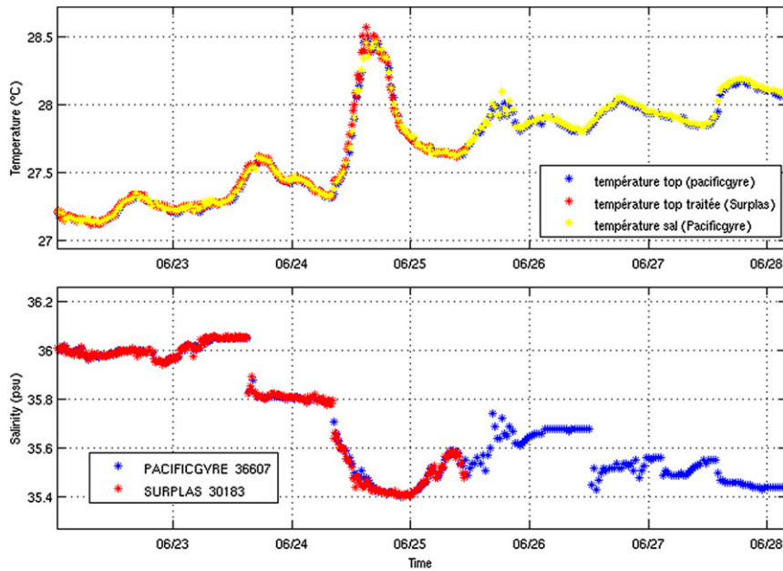
FIG. A1. Zoom in the time series from PG36607 and Surplas 30183 in June 2011, near 2°N, 32°W (UTC time). (top) T ; (bottom) S (red, for Surplas, and blue for PG data).
