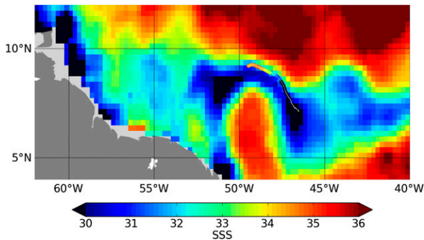
FIG. B2. As in (bottom) in Fig. B1 for a short period (11–20 Sep 2011) of the trajectory of drifter PG73226. Drifter is entrained in the retroflexion of the North Brazil Current, probably on its outer rim.
