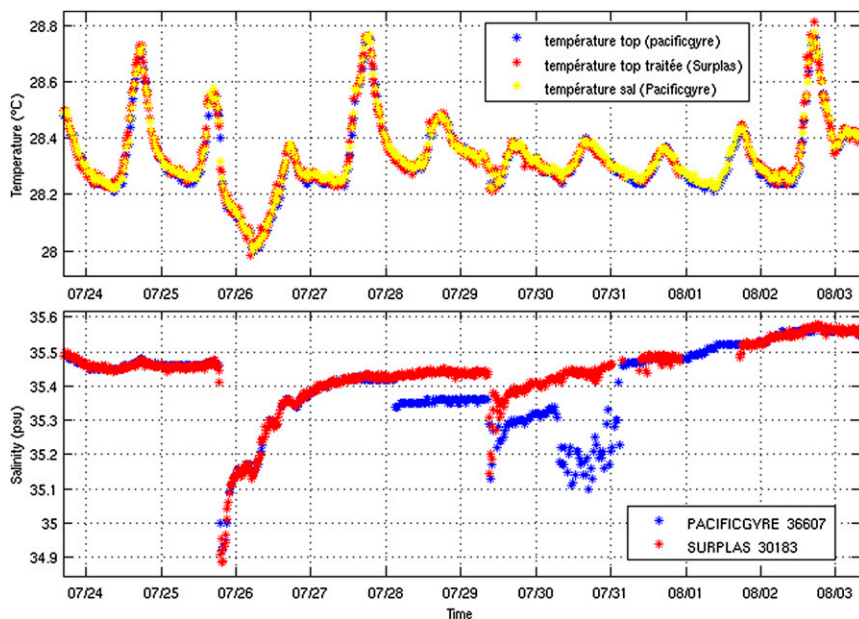
FIG. A2. Time series from drifter PG36607 and its attached Surplas 30183 deployed in 2011 in the equatorial Atlantic: (top) T and (bottom) S (red, for Surplas, and blue for PG data).
