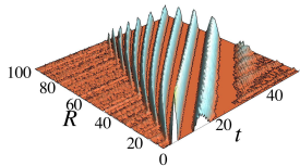
(b1) \alpha=1/2
