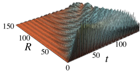
(a2) \alpha=3/2
