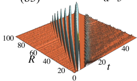
(b3) \alpha=3
