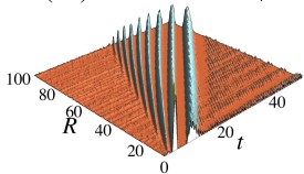
(b2) \alpha=3/2
