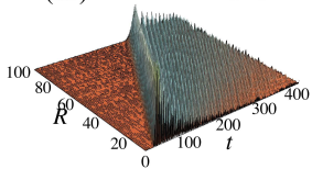
(a3) \alpha=3
