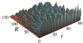
(a1) \alpha=1/2
