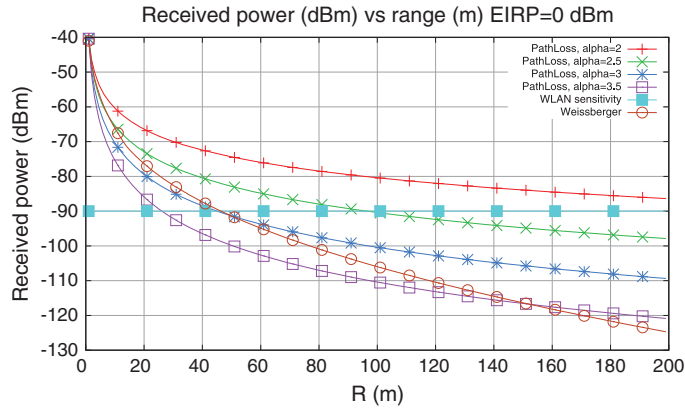
Figure 2. Received power versus distance for the Weissberger and path loss models ( \alpha = 2, 2.5, 3, \text{ and } 3.5 ) considering a 0 dBm transmitted power.
