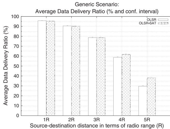
Figure 4. Generic scenario: data delivery ratio for OLSR and OLSR-SAT as a function of the distance between source and destination (95% confidence interval).
