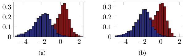
Fig. 15. Histograms of the similarity measure \log(\delta_W) for \hat{K}^* = \hat{K} and \hat{K}^* = \hat{K} + 1 . The blue and red bins correspond to the changed and unchanged areas, respectively. (a) Histogram of \log(\delta_W) for \hat{K}^* = \hat{K} (no overestimation). (b) Histogram of \log(\delta_W) for \hat{K}^* = \hat{K} + 1 .
