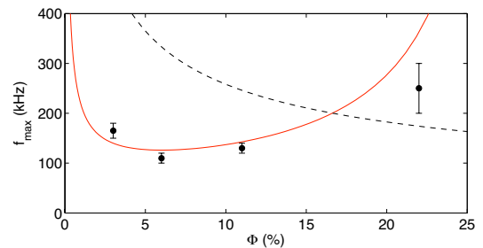
FIG. 2: Frequency of the maximum of attenuation as a function of the liquid fraction, for median radii of 40\mu\text{m} . Dashed line is the Minnaert resonance frequency with an effective density: f_M/\sqrt{\Phi} . Solid line is the prediction of our model.
