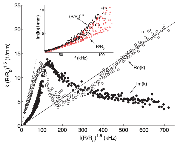
FIG. 3: Rescaled dispersion relation for a reference median radius of R_0 = 40\mu\text{m} . Lines are for constant velocities of 32 (dash) and 220 m/s (solid). Inset: the R^{-1.5} scaling (solid symbols) is better than the R^{-1} one (open symbols).
