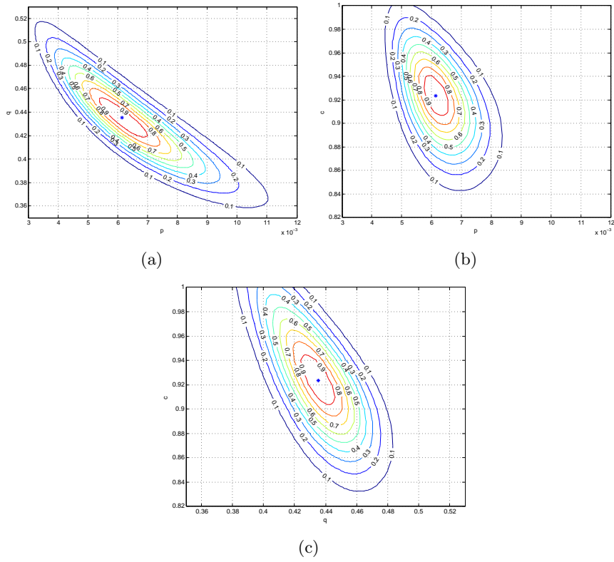
Figure 5: Contour plots of pI_{\mathbf{x}}(\theta) in two-dimensional parameter subspaces with (a): c = \hat{c} , (b): q = \hat{q} (b) and (c): p = \hat{p} .
