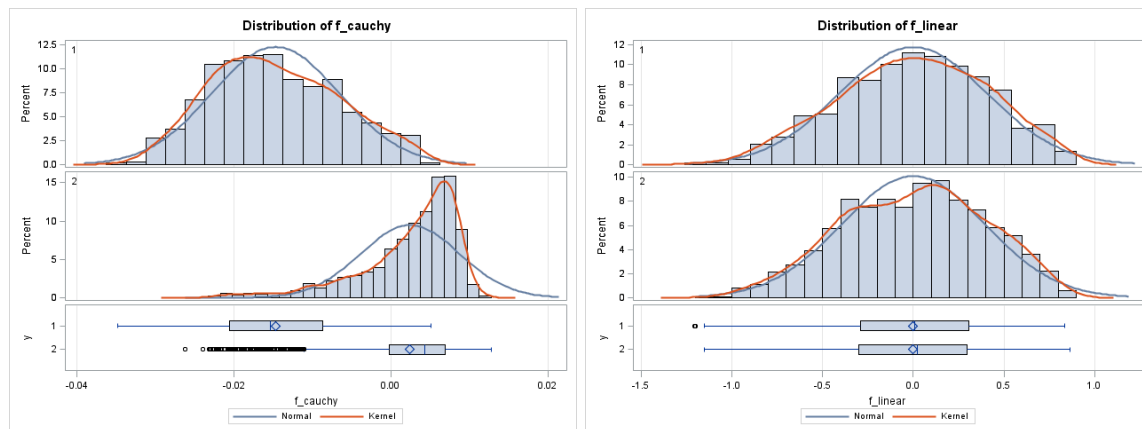
Figure 1: 2-classes distributions
