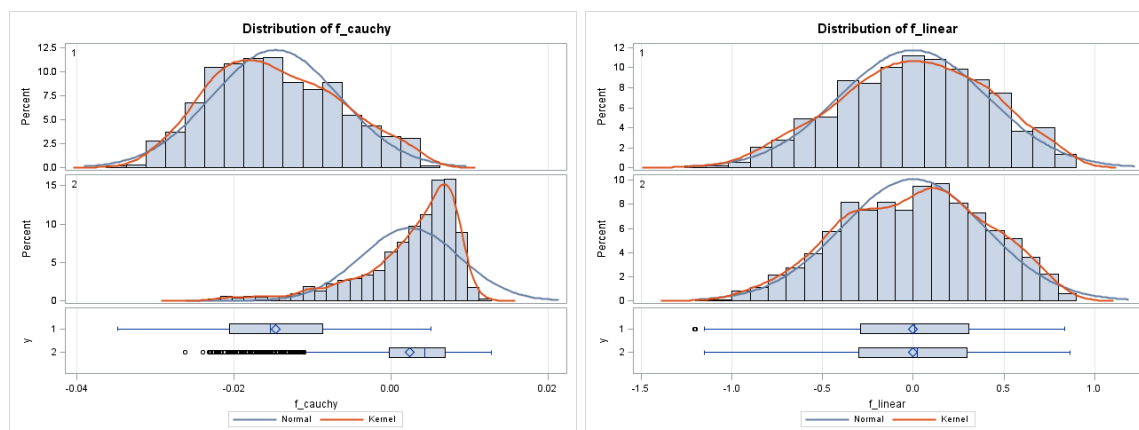
Figure 1: 2-classes distributions
