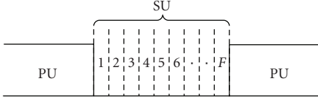
FIGURE 5: Single-user case with F subcarriers in one spectrum hole.
