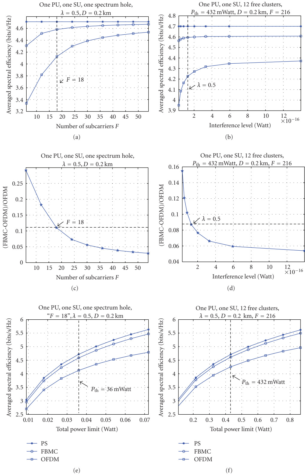
FIGURE 7: Experimental results of single-user resource allocation for one and multiple spectrum holes with D = 0.2 km: (a) Averaged spectral efficiency versus number of subcarriers for one spectrum hole case. (b) Averaged spectral efficiency versus interference level for multiple spectrum holes case. (c) (FBMC-OFDM)/OFDM versus number of subcarriers for one spectrum hole case. (d) (FBMC-OFDM)/OFDM versus interference level for multiple spectrum holes case. (e) Averaged spectral efficiency versus total power limit for one spectrum hole case. (f). Averaged spectral efficiency versus total power limit for multiple spectrum holes case.
