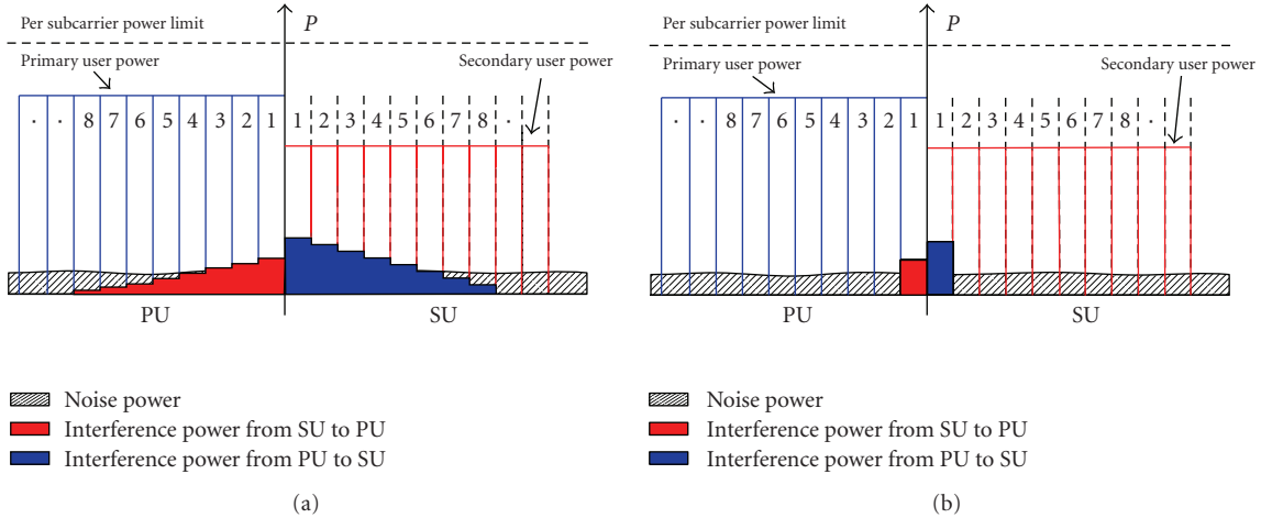
FIGURE 3: (a) Intercell interference between PU and SU in OFDM based CR networks (b) Intercell interference between PU and SU in FBMC based CR networks.
