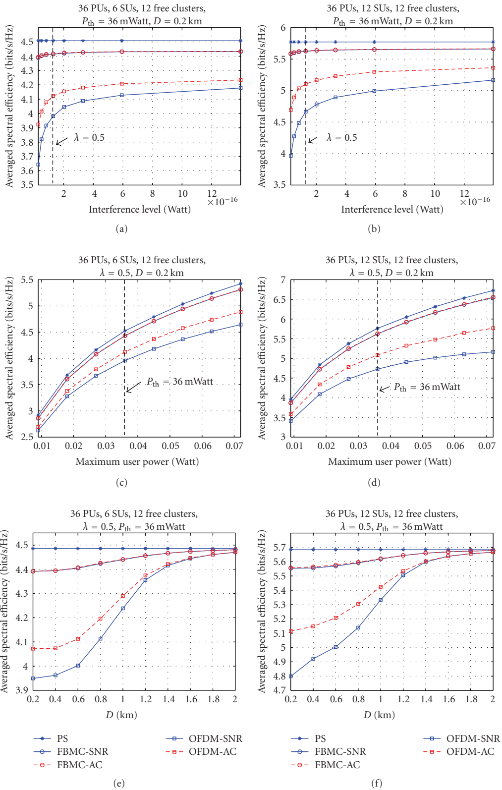
FIGURE 8: Experimental results of Multiuser resource allocation for multiple spectrum holes with F = 216 : (a) Averaged spectral efficiency versus interference level for 6 SUs. (b) Averaged spectral efficiency versus interference level for 12 SUs. (c) Averaged spectral efficiency versus maximum user power limit for 6 SUs. (d) Averaged spectral efficiency versus maximum user power limit for 12 SUs. (e) Averaged spectral efficiency versus distance between SBS and PBS for 6 SUs. (f) Averaged spectral efficiency versus distance between SBS and PBS for 12 SUs.
