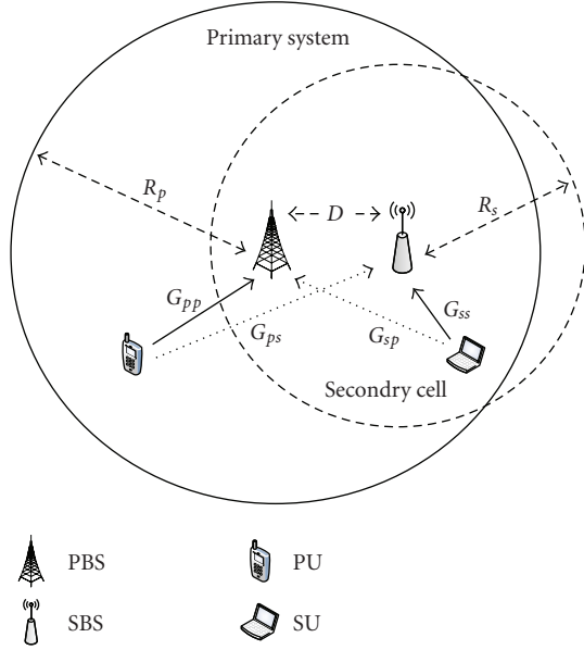
FIGURE 1: Cognitive radio networks with one primary system and one secondary cell.
