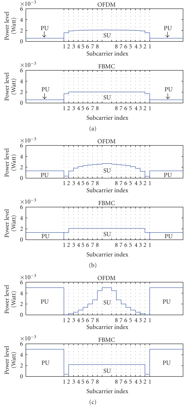
FIGURE 6: Three typical channel realizations of single-user case with F = 18 , \lambda = 0.5 , D = 0.2 km, and P_{th} = 36 mWatt: (a) D_{SU-SBS} > D_{PU-PBS} (b) D_{SU-SBS} \approx D_{PU-PBS} (c) D_{SU-SBS} < D_{PU-PBS} .
