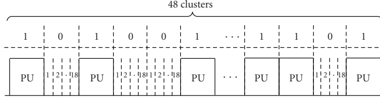
FIGURE 2: Distributions of the primary users and the spectrum holes with “ N_{\text{all}} = 48 ” and L=18 .
