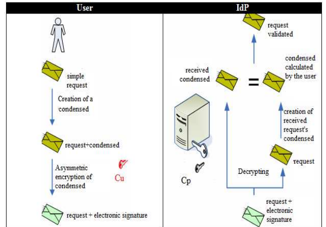
Figure 3: Encryption technique
