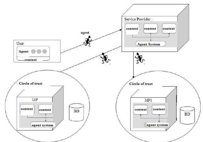
Figure 2: Agent System
