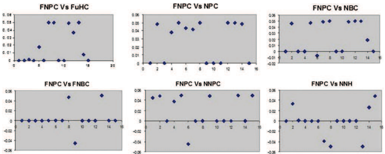
Fig. 2 Results of the paired t test between the FNPC and other classifiers
