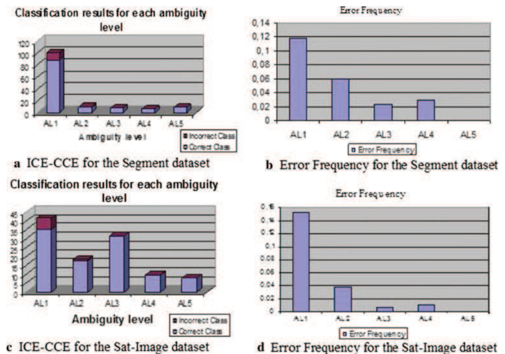
Fig. 4 Results for the NNPC
