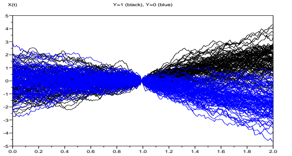
Fig. 2. Sample of size n = 100 for each class of Y .
