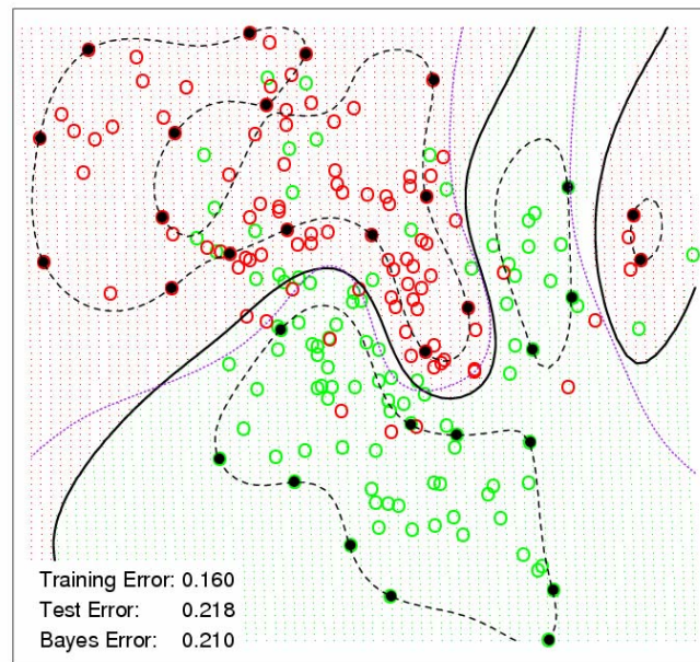
SVM - Radial Kernel in Feature Space
