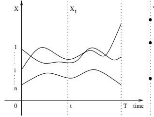
Figure 1: Regression on a stochastic process
