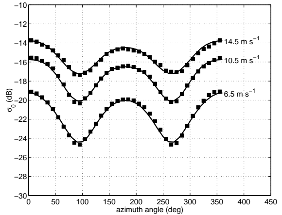
Figure 2: Azimuthal modulations of QSCAT measurements estimated for three wind speed for the vertical polarization. The square show the bin-averaged mean of \sigma_0 . The full line shows the QSCAT-NN model.
