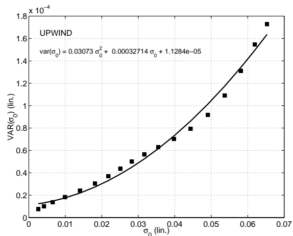
Figure 4: The estimated variance by the neural model with respect to the estimated mean of \sigma_0 by QSCAT-NN model for the vertical polarization and the upwind direction. This relationship has a quadratic form.
