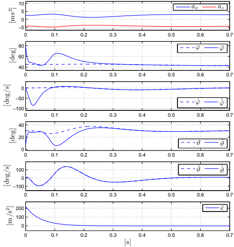
(c) Observer Results: zoom on the first 0.7 seconds of simulation. The remaining part is not displayed because the observer follows the state with high fidelity. \hat{\varphi} and \dot{\hat{\varphi}} are always equal because the estimated value comes from the direct measure of the gyroscope. The prediction error does not increase even when the tension goes to zero for an instant.
