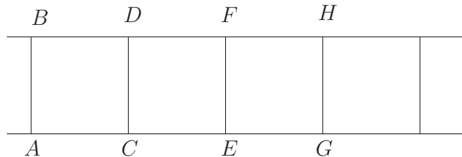
FIGURE 8. At the points A and B and at the points C, E, G, \dots the angles are right. Under the second hypothesis, the segments CD, EF, GH, \dots decrease more than linearly with respect to the distances from the points C, E, G, \dots to the point A . Likewise, the more the angle at D, F, H, \dots is far, the more obtuse it is.
