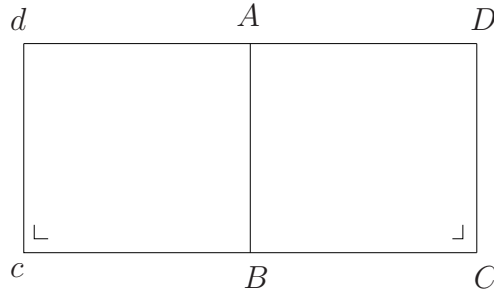
FIGURE 7. The isosceles birectangular quadrilateral cCDd is obtained by folding the trirectangular quadrilateral ABCD along the side AB . The angles at c and C are right and cd = CD .
