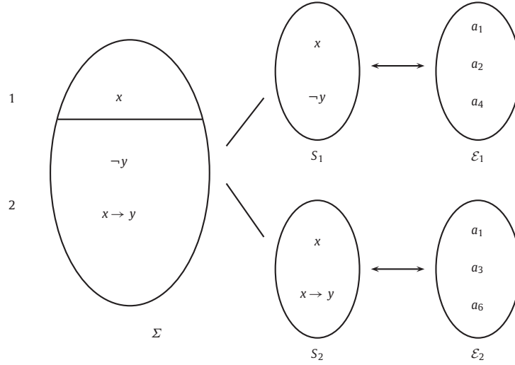
Fig. 1. Preferred sub-theories of \Sigma vs. stable extensions of (\text{Arg}(\Sigma), \text{Undercut}, \succcurlyeq_{WLP}) .
