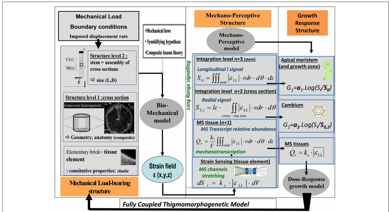
FIGURE 10 | Schematic representation of thigmomorphogenetic model including the ISM beam model and the S 3 m.
