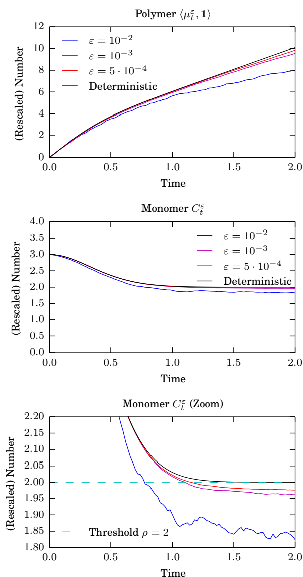
FIG 4. Case Id) constant rate coefficients a and b with initially incoming characteristics (see Table 1). We plot the time evolution of the total number of clusters \langle \mu_t^\varepsilon, 1 \rangle (top) and the number of particles C_t^\varepsilon (middle and down) for different \varepsilon (see legend), together with the deterministic solution of the moment equations (50) (in black). The moment equations give a very good approximation of the stochastic solution. Down, we zoom around the value \rho = 2 and illustrate the fact that C_t^\varepsilon crosses the threshold \rho in finite time, while the deterministic limit c_t does not. We also observe that the deterministic approximation is slightly worst after the time C_t^\varepsilon crosses the threshold \rho .
