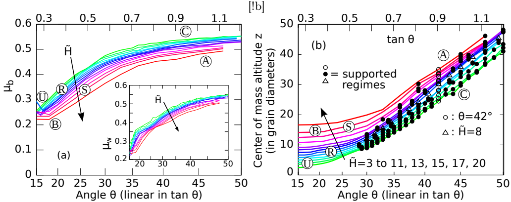
FIGURE 4. (a) Effective friction coefficients on the base \mu_b and the wall \mu_w (inset) as a function of the inclination angle \theta . Both coefficients increase with \theta but show a reduction for increasing mass hold-up. (b) Altitude of the center of mass C_M as a function of \theta for various mass hold-up. Markers indicate the states corresponding to the supported flow regimes for which C_M exhibits a linear increase with \tan \theta . Labels U, R, C, A, S and B refer to the different flow regimes defined in Fig. 6.
