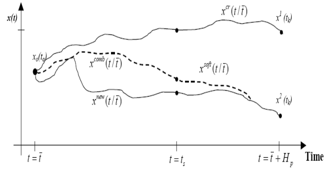
Fig. 6. Soft switching.
