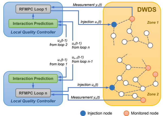
Fig. 12. Structure of distributed RFMPC.
