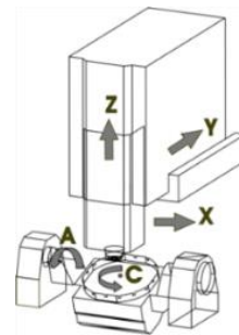
FIGURE 4. MACHINE-OUTIL CINQ AXES MIKRON UCP 710.
