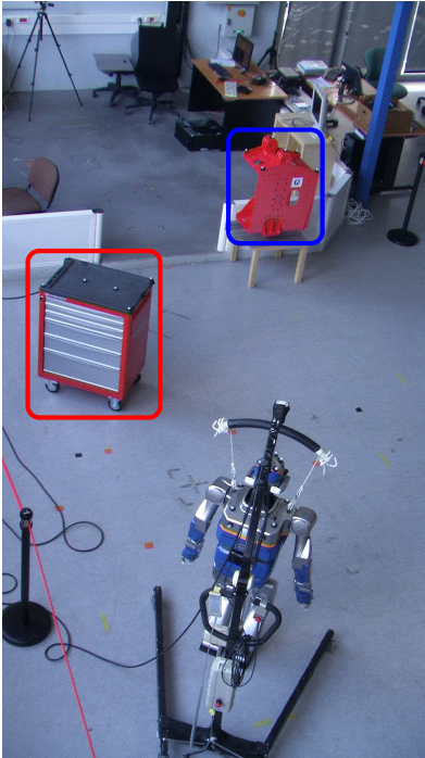
Fig. 1. Situation of the experiment: The robot has to go in the vicinity of the pylon engine depicted in blue while avoiding the red moving toolbox
