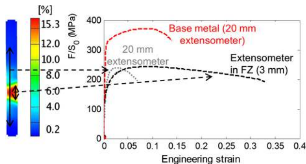
Fig. 1—Nominal stress–strain curves of the base material and of the transverse weld assembly. The map of plastic deformation as measured for the weld assembly by digital image correlation is shown. The two nominal stress–strain curves for the weld are obtained using respectively a gauge length of 3 mm within the fusion zone and of 20 mm across the different weld zones.
