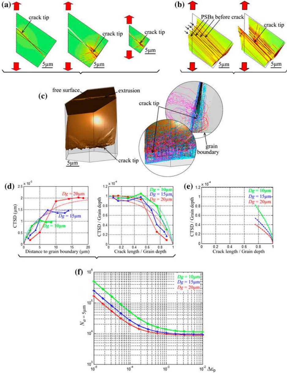
Figure 5. (colour online) (a) Von-Mises strain field for different crack front positions (from the grain boundary) and for 20 and 10 μm grain depths. (b) Von-Mises strain field at higher imposed plastic strain ( 5 \times 10^{-4} ), before and after crack introduction. The displacement field is magnified \times 30 for clarity. (c) Crack front morphology and associated dislocation microstructure. (d) CTSD evolution as a function of the crack tip position for the three different grain depths, evaluated using Equation (3). (e) CTSD evolution as a function of crack tip position for the three tested grain depths, evaluated using Equation (2). (f) Number of cycle to get a 5 μm length crack, evaluated using Equation (4).
