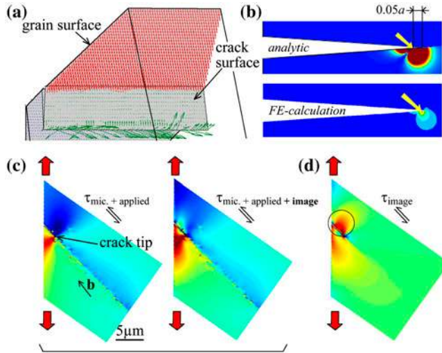
Figure 8. (colour online) (a) Traction vector acting in the different free surfaces. (b) Von Mises stress field evaluated using analytical (using point forces [34]) and FE calculation solutions. Good accuracy of the analytical solution, including in the vicinity of the crack tip, can be noticed. (c) Stress field (shear component on the primary slip plane) calculated without and with image forces. (d) Image stress field acting in the simulated grain.
