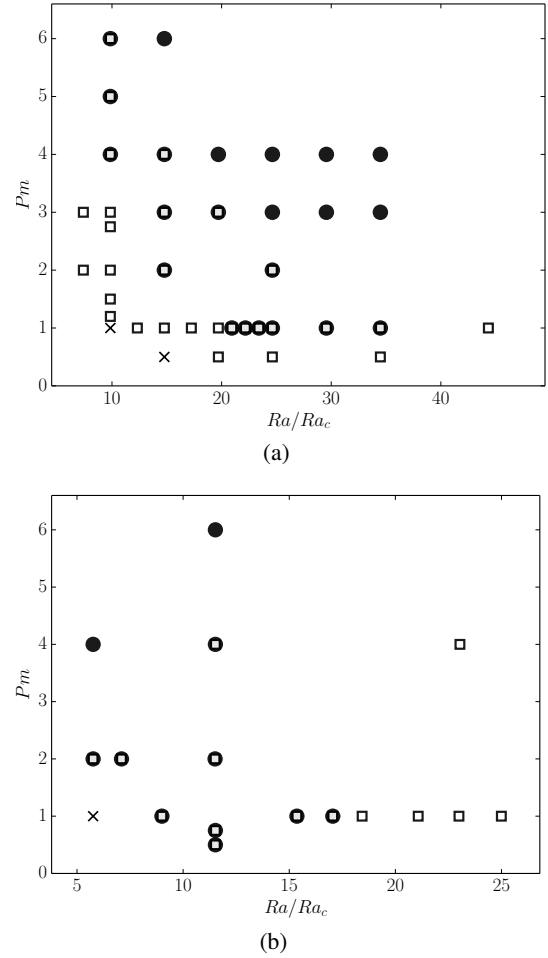
Fig. 1. Dipolar (black circles) and multipolar (white squares) dynamos as a function of Ra/Ra_c and Pm , for a central mass a) and a uniform mass distribution b) . Crosses indicate the absence of a self-sustained dynamo.
