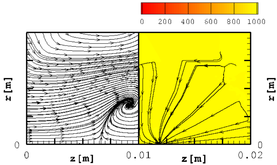
Figure 10: Pathlines in the solid (left) and the fluid (right) and fluid density at t = 40.0 \mu\text{s} .
