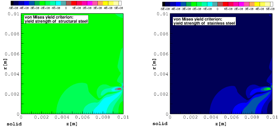
Figure 20: Evaluation of simplified yield criterion for structural steel (left) and stainless steel (right) at t = 56.0 \mu\text{s} .
