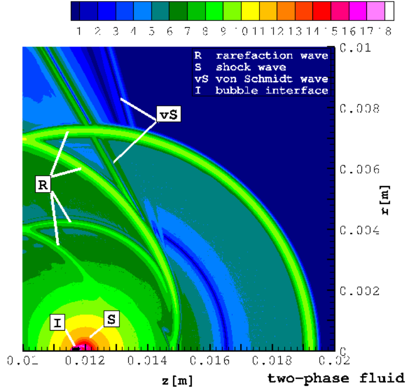
Figure 9: Density gradient magnitude (logarithmic scaling) at t = 40.0 \mu\text{s} .
