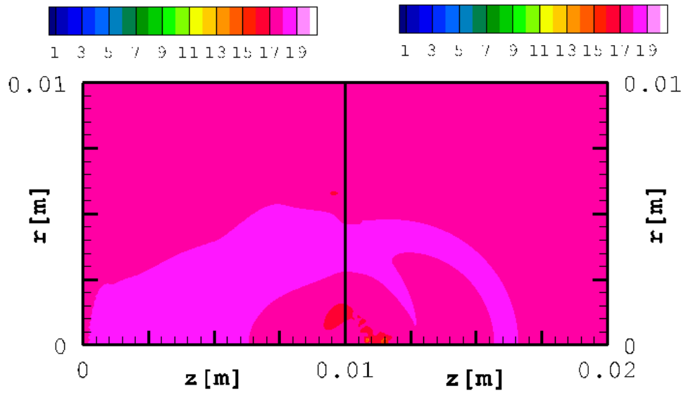
Figure 16: Logarithm of the absolute values of the stress component \bar{\sigma}_{zz} in the solid (left) and the pressure in the fluid (right) at t = 65.7 \mu s .
