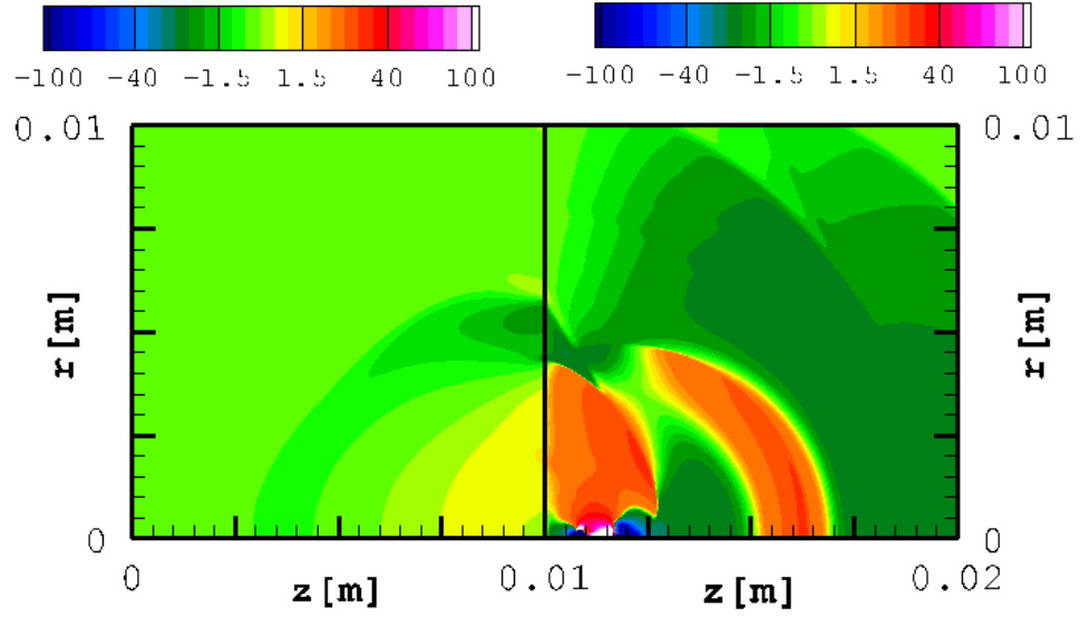
Figure 15: Velocity component v_z in the solid (left) and the fluid (right) at t = 65.7 \mu s .
