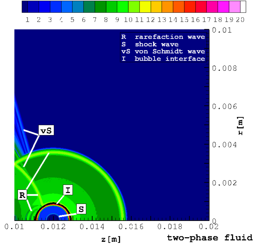
Figure 5: Density gradient magnitude (logarithmic scaling) at t = 16.6 \mu s .
