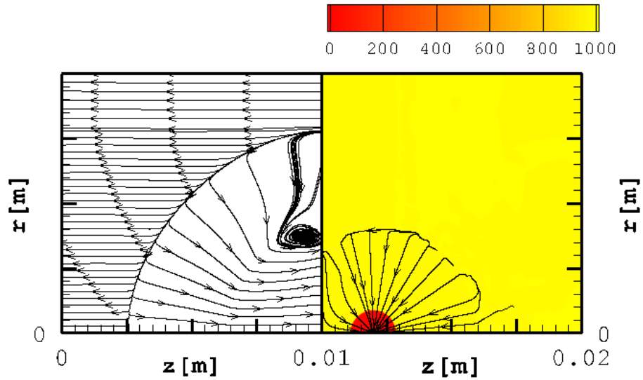
Figure 6: Pathlines in the solid (left) and the fluid (right) and fluid density at t = 16.6 \mu s .
