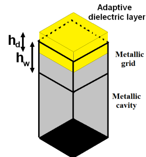
Fig. 9. Schematic representation of the square metallic waveguide with the matching dielectric layer. h_w=20\text{mm} , h_d=12\text{mm} .
