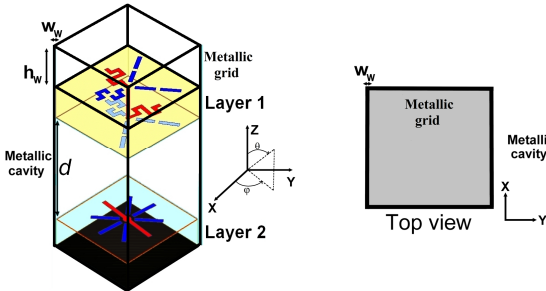
Fig. 7. Schematic representation of the square metallic cavity. The four edges of the cell are PEC walls forming a metallic cavity: w_w=0.1\text{mm} , h_w=20\text{mm} .
