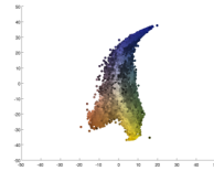
(e) Chromaticity diagram of 2b.
