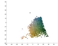
(f) Chromaticity diagram of 2c.
