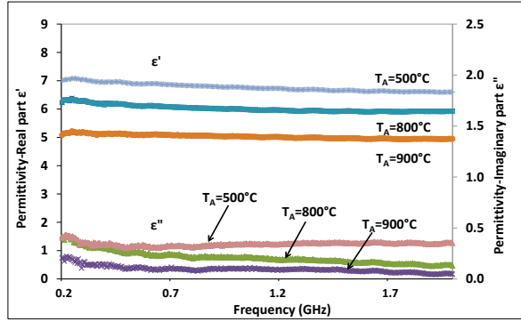
Fig.3. Complex permittivity spectra for samples S1 ( T_A=500^\circ\text{C} ), S2 ( T_A=800^\circ\text{C} ), S3 ( T_A=900^\circ\text{C} ) over the frequency range 0.1-6 GHz.
