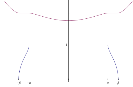
FIGURE 8. The density of the minimising measure \mu_T^* and the graph of the function x \mapsto U^{\mu_T^*}(x) + \frac{T}{4}x^2 , for T slightly larger than 14.
