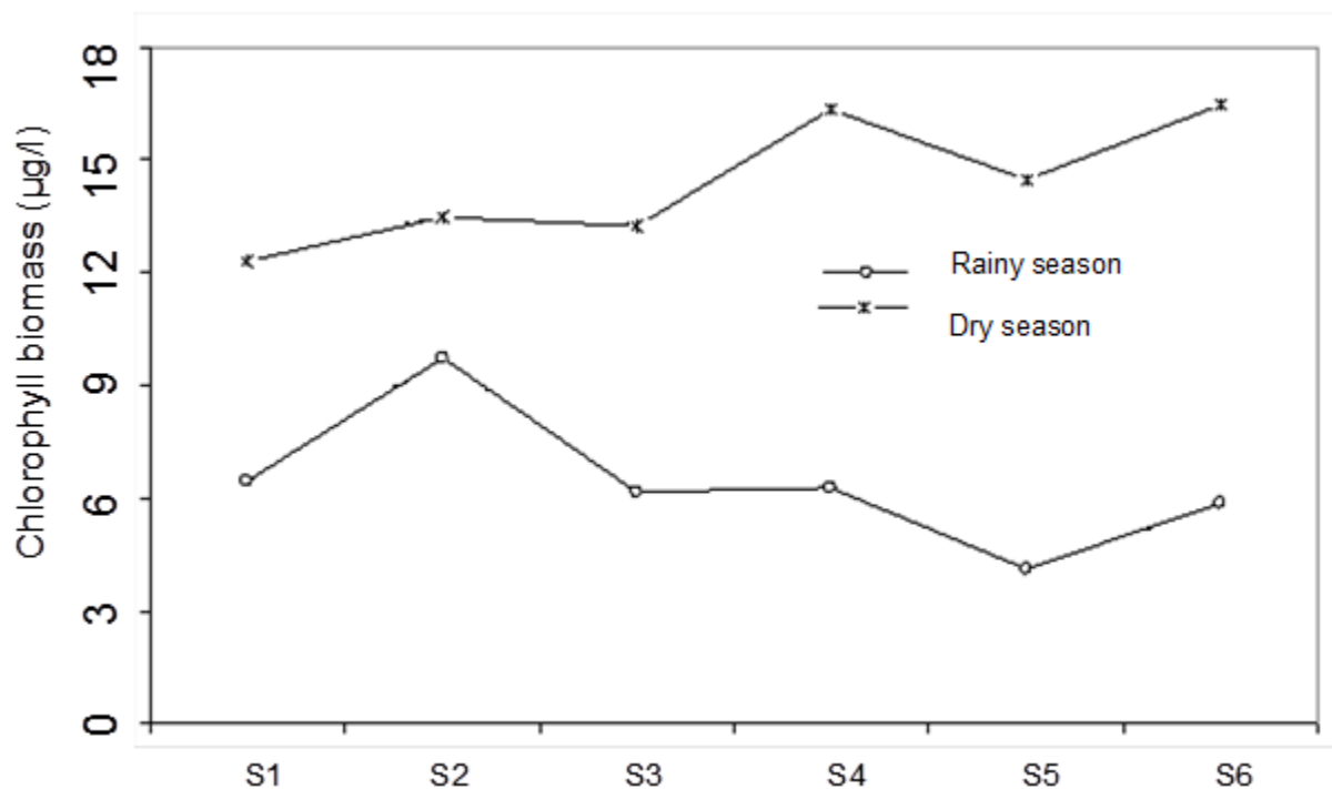
Figure 6: Annual change in total biomass Chlorophyll ( \mu\text{g} / \text{l} ) in the six stations of Lake Taabo for flood periods (= rainy season from June to October) and low water (= dry season from December to March).
