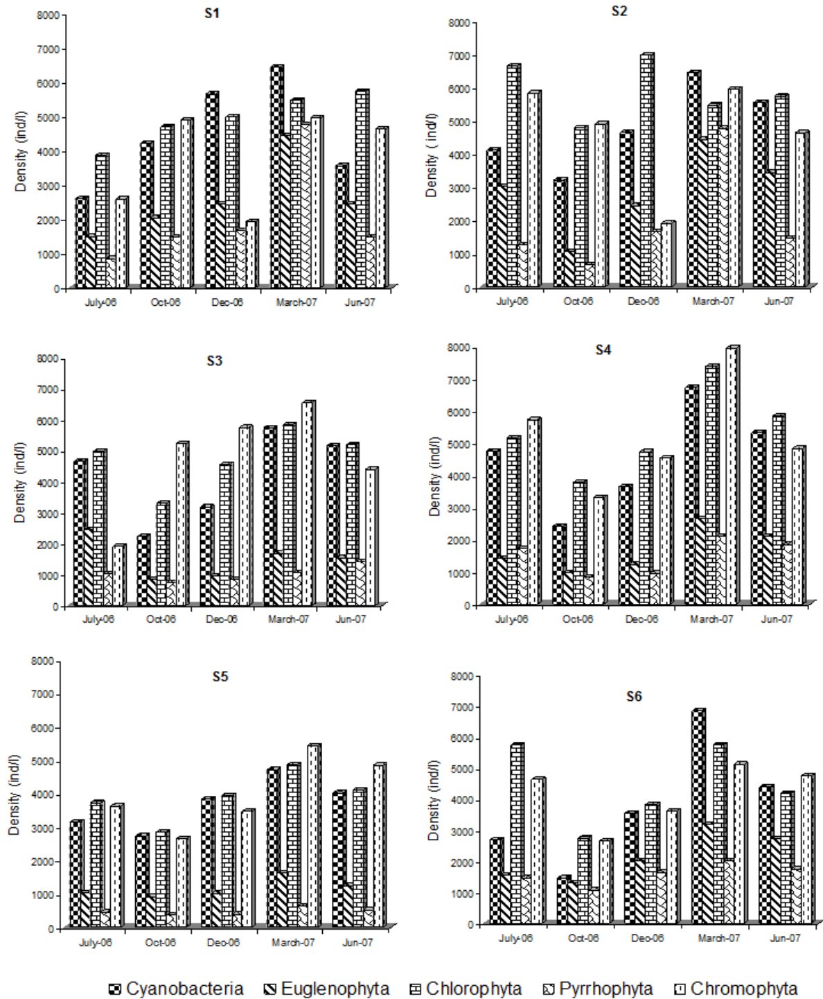
Figure 3 : Distribution of the phytoplankton density in different stations
