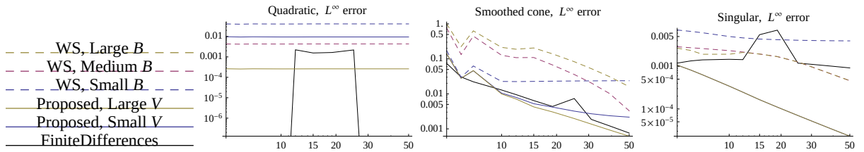
Figure 3: Log-Log plot of the L^\infty error, as a function of resolution n , for the three test cases. Discretization set X \subseteq \Omega has n^3 points. Scheme stencils on Figure 1.
