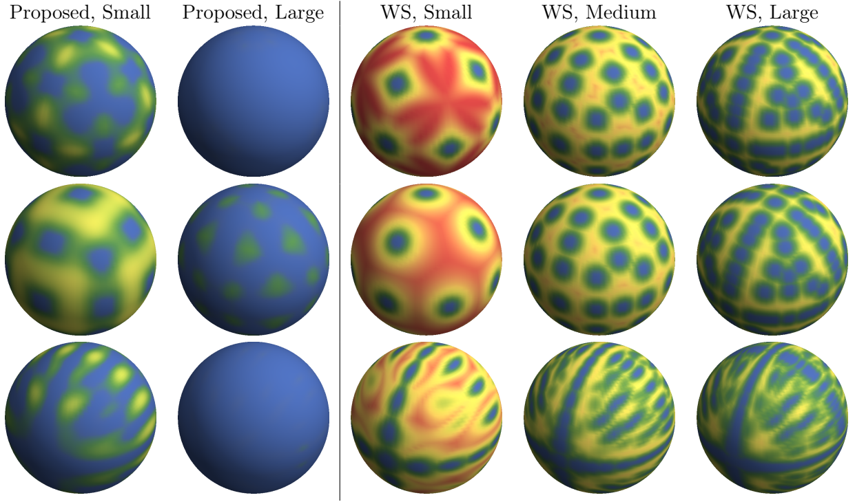
Figure 2: Relative consistency error (\mathcal{D}u_M - \det(M))/\mathcal{D}u_M (blue = 0, red = 1) for a quadratic (8) map u_M associated to a matrix M = M(v) , with v in the unit sphere (hence the spherical plot). First line: M(v) has eigenvalues 6^2, 1, 1 , the former with eigenvector v . Second line likewise with eigenvalues 6^{-2}, 1, 1 . Third line M(v) = R(v)DR(v) where R(v) is the rotation of axis v and angle \pi , and D is diagonal of entries 6, 1, 1/6 .
