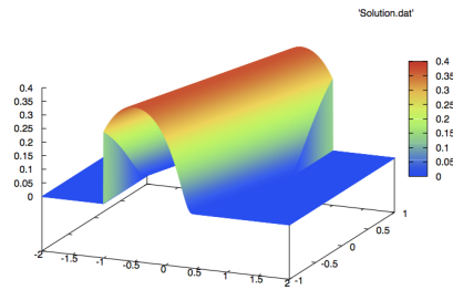
Solution for k = 1
