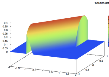
Solution for k = 3
