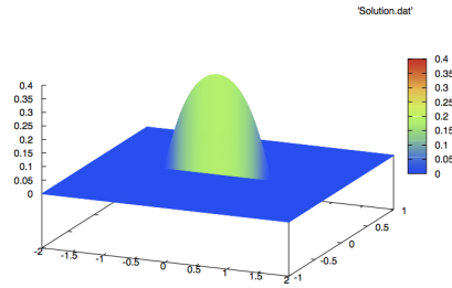
Solution for k = 400
