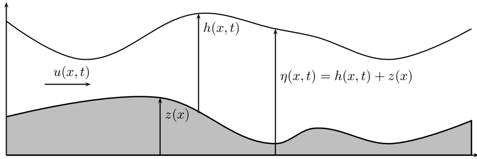
Figure 1: Non conservative variables for SWE equations.
