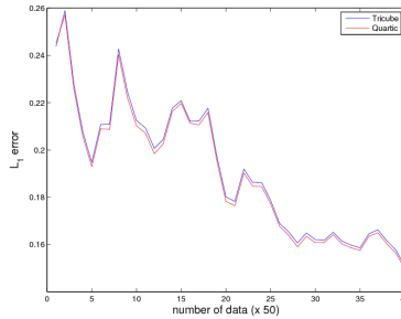
Fig. 1. Consider a law X whose density in the tangent plane at (0,0) is a centered hemisphere. From a set of draws, the density is estimated using two standard kernels, K(x) = (1 - x^2)^2 \mathbf{1}_{x < 1} and K(x) = (1 - x^3)^3 \mathbf{1}_{x < 1} . The L_1 distance between the estimated and the true density is plotted depending on the number of draws.
