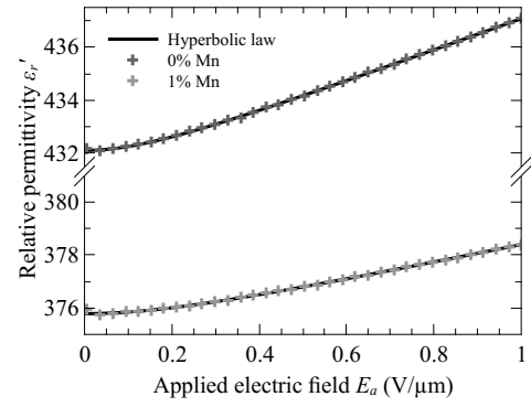
Figure 7. Examples of the hyperbolic law fits at 10 kHz for undoped BST and for a 1% manganese dopant rate.
