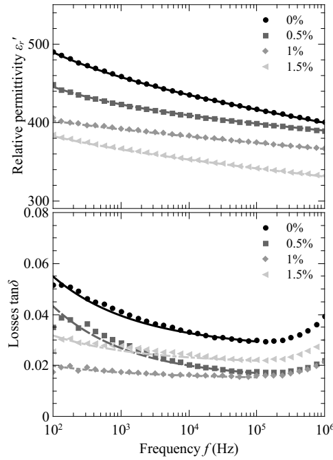
Figure 6. Relative permittivity and dielectric losses as a function of frequency for the different manganese dopant rates. The increase of the losses above 10^5 Hz is artificial and due to a resonance of the impedance analyzer.
