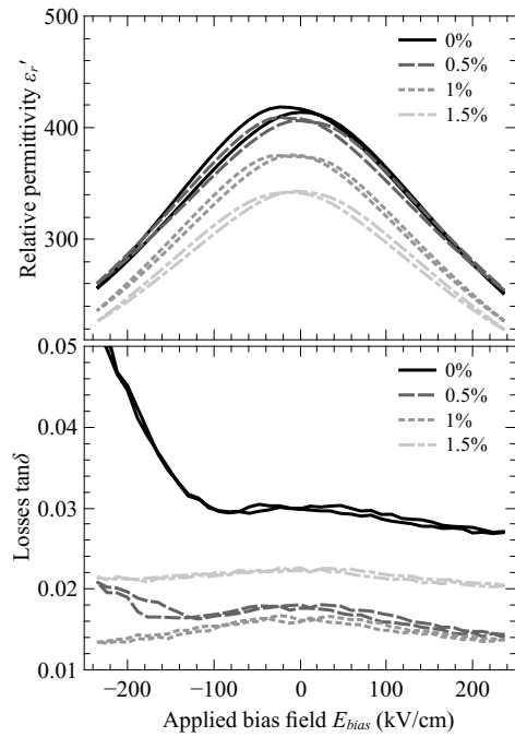
Figure 4. Relative permittivity and losses as a function of the applied bias field at 100 kHz for the different manganese dopant rates.
