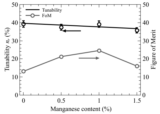
Figure 5. Tunability and figure of merit under 235 kV/cm at 100 kHz and as a function of the manganese content.
