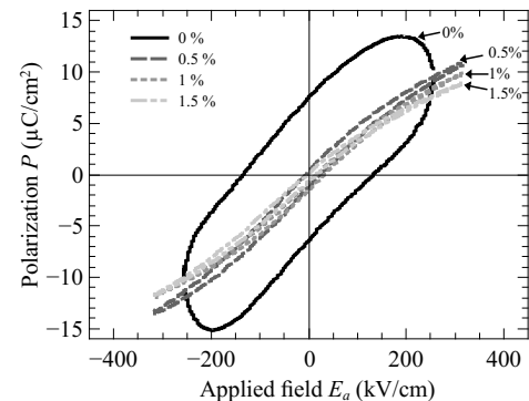
Figure 3. Hysteresis loops of the BST(80/20) films with different manganese dopant rates.
