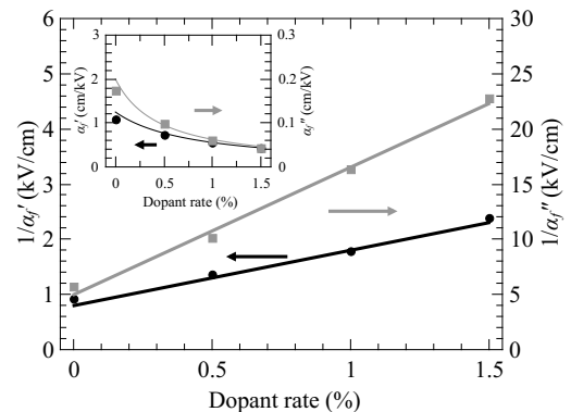
Figure 9. Inverse of the coefficients \alpha'_f and \alpha''_f obtained by fitting of the irreversible part of the permittivity.
