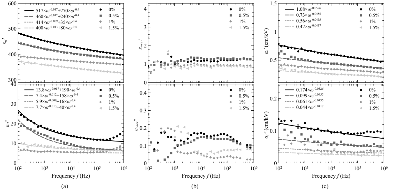
Figure 8. Real and imaginary part of the permittivity as a function of frequency, decomposed according to the hyperbolic law, showing the bulk contribution (a), and the contributions of domain wall vibrations (b) and domain wall displacements (c). The increase of the imaginary part above 10^5 Hz is artificial and due to a resonance of the impedance analyzer.
