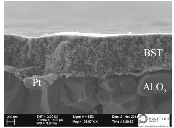
Figure 2. Typical cross section micrograph of the BST(80/20) thin films.
