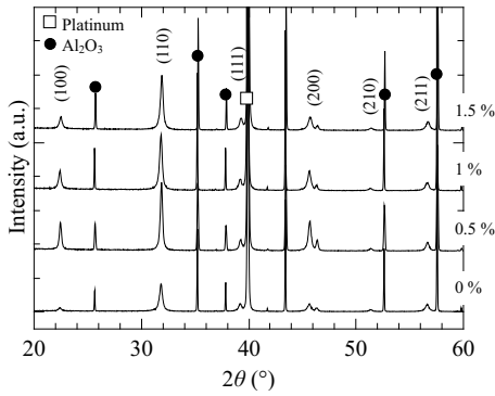
Figure 1. X-ray diffraction patterns of the BST(80/20) thin films on platinum coated alumina substrates for the different manganese dopant rates.
