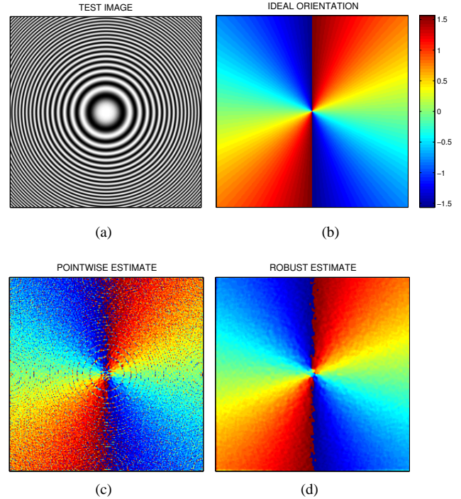
Fig. 1. Monogenic orientation estimate in the presence of noise. (a) noise-free test image containing a full 360-degree range of orientations. (b) ideal orientation. (c-d) pointwise and robust ( \sigma = 2 ) estimates in the presence of image noise (20 dB). Mean square error of the estimate is 1.2E-2 for (c) and 2.7E-4 for (d). Phases are wrapped in the [-\pi/2, \pi/2] interval.
