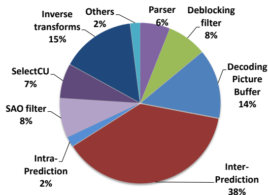
Fig. 4: Actors workload of the HEVC decoder
