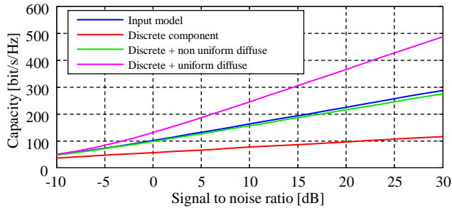
Fig. 7. Water filling channel capacity: Model and its estimate
