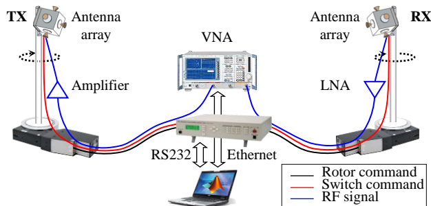
Fig. 1. Overview of the UWB channel sounder
