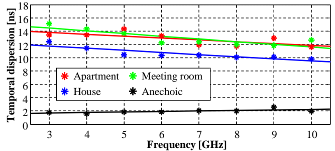
Fig. 14. Delay spread parameter versus frequency
