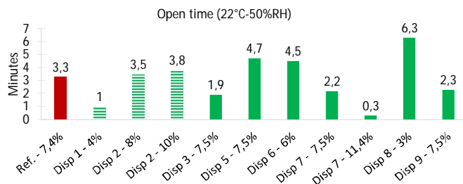
Fig.3: Open time - Weight ratio % (commercially available dispersant/pigments and fillers)
