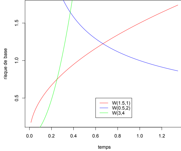
Figure 1 – Plots of the baseline hazard function for different parameters of a Weibull distribution \mathcal{W}(a, \lambda)
