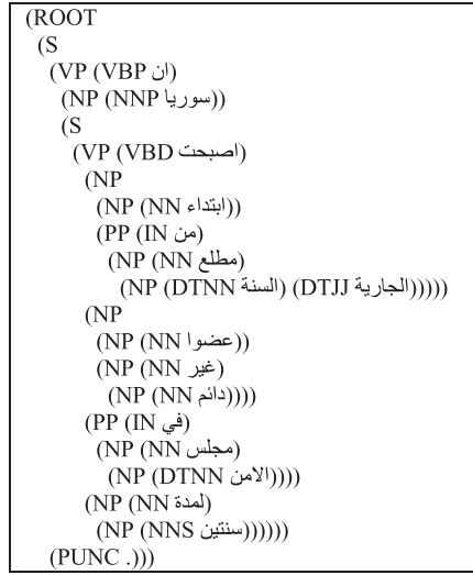
Fig. 2. Syntactic analysis of the example (4) as given by ATB manual annotations.
