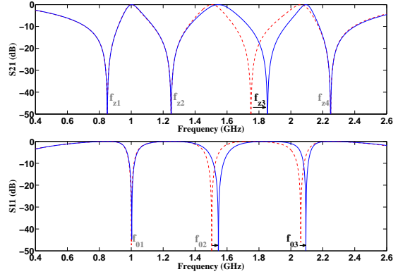
(b) Variation of C_3 from 1.042 pF (red dashed lines) to 0.896 pF (blue solid lines), C_1 = 3.415 pF, C_2 = 1.998 pF and C_4 = 0.506 pF in both cases.
