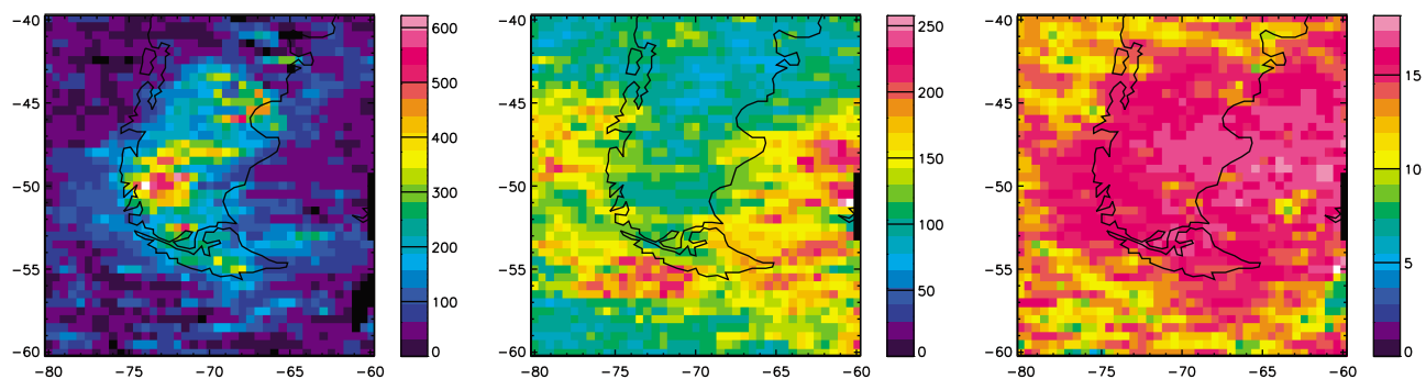
Figure 9. Results of the AIRS imagery analysis plotted versus longitude and latitude, showing (left) momentum flux (mPa), (center) horizontal wavelength (km), and (right) vertical wavelength (km).
