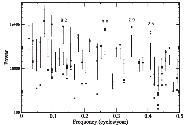
FIG. 13. Spectral analysis of the atmospheric model's combined barotropic and baroclinic modes using MSSA. The MC MSSA spectrum shown is computed with window width M = 150 months; other details as in Figs. 5 and 9.
