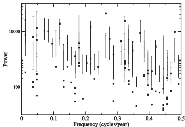
FIG. 21. Spectral analysis of the atmospheric model's combined barotropic and baroclinic modes, but when the model is driven by a spatially smoothed SST field; see text for details. MC MSA spectrum computed with window width M = 150 months, same conventions as in Figs. 9 and 13.
