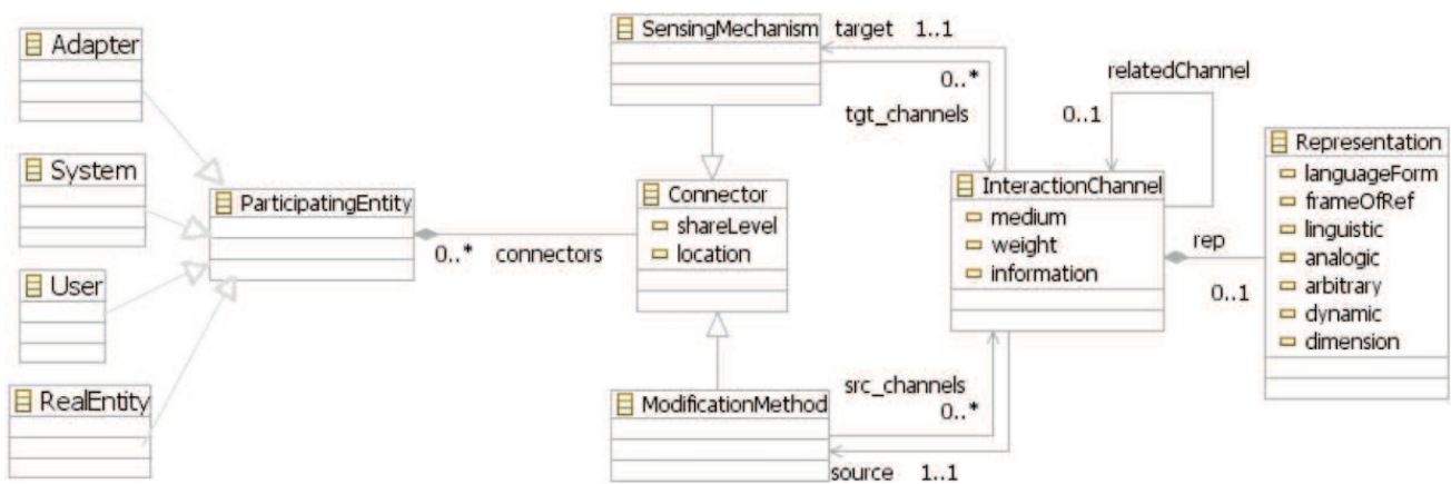
Fig. 8. Main elements of the ASUR metamodel.
